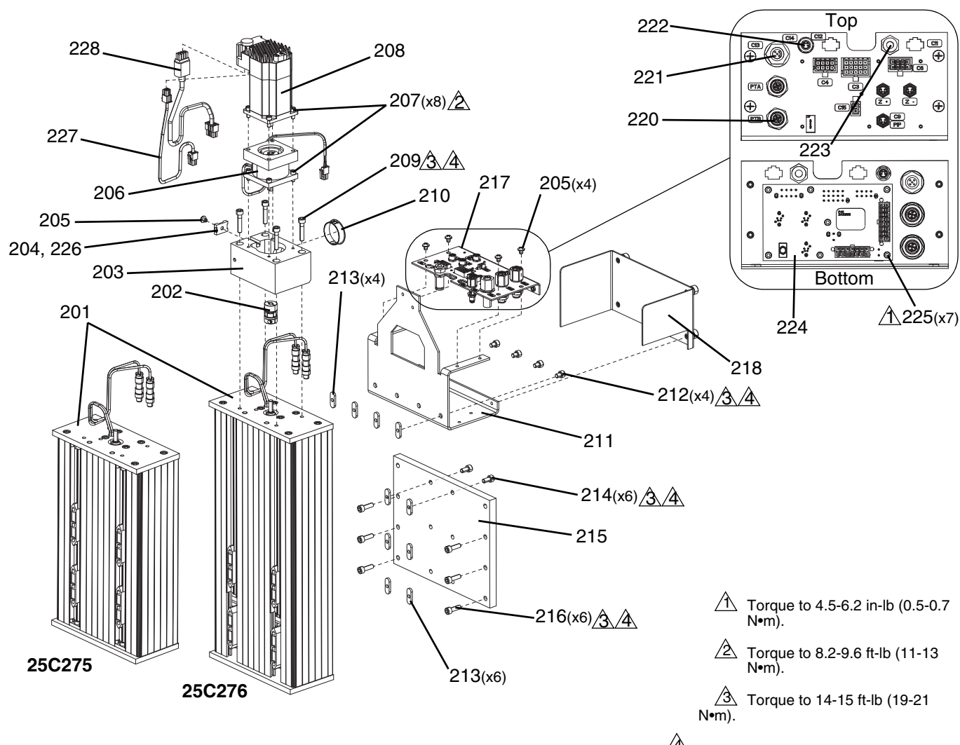
FIG. 11: Axis Z Actuators
