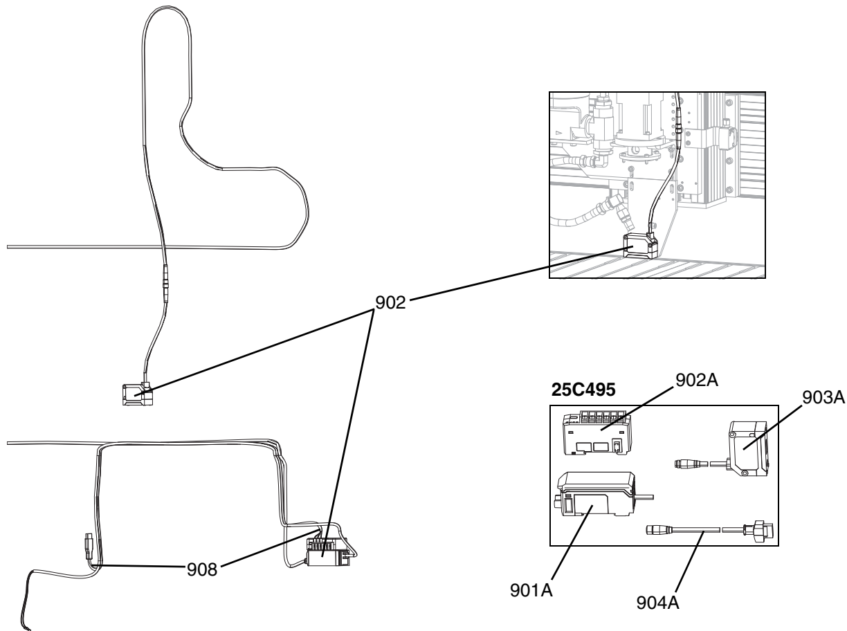
FIG. 30: Z-Height Sensor Kit
