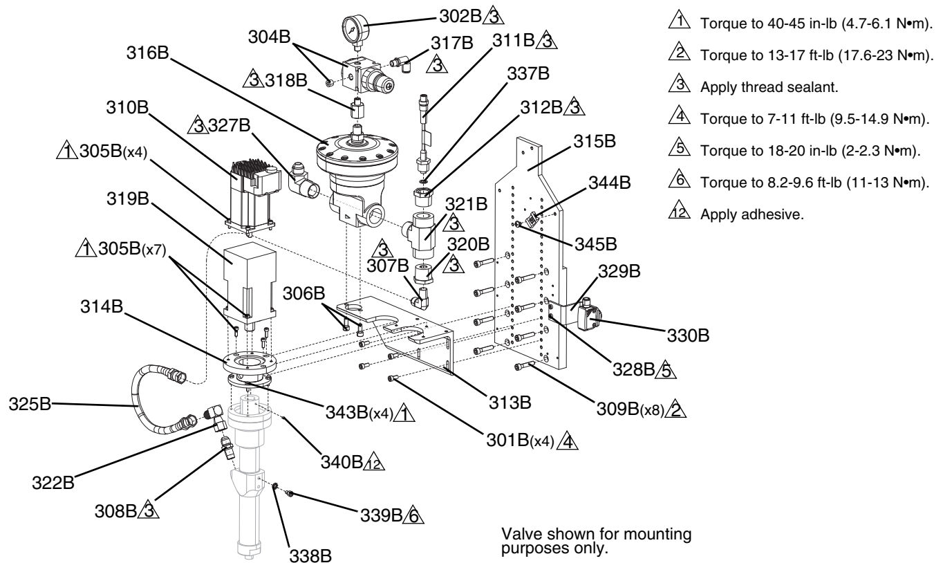
FIG. 15: PC Pump Valve Holder
