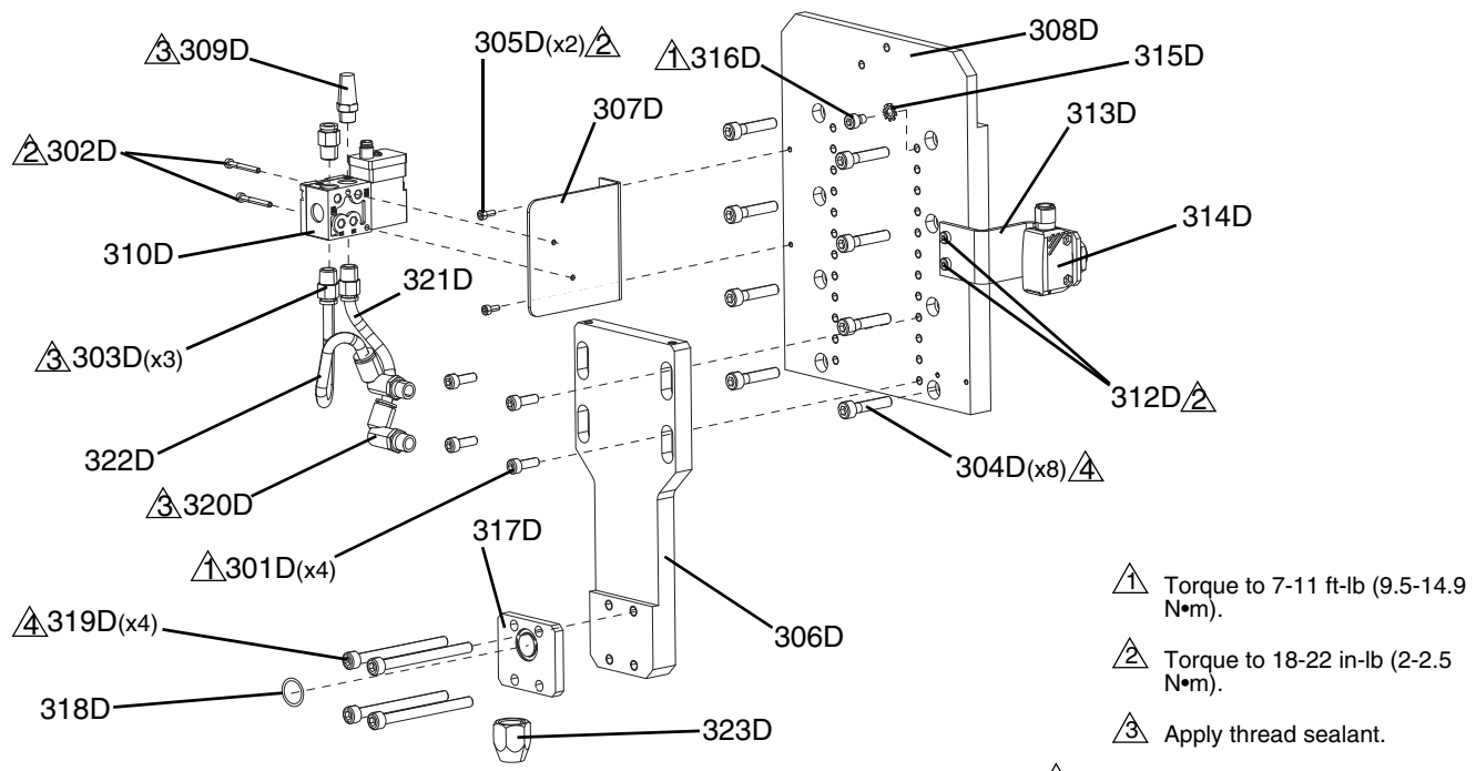
FIG. 17: Ambient Endure Valve Holder
