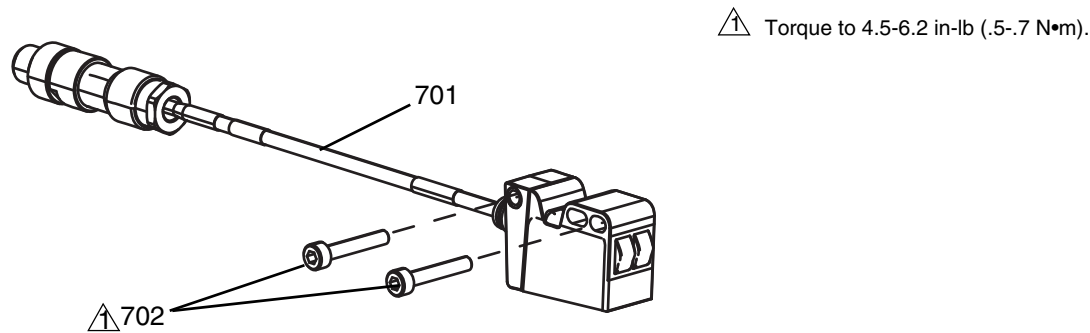
FIG. 28: Part In Place Sensor
