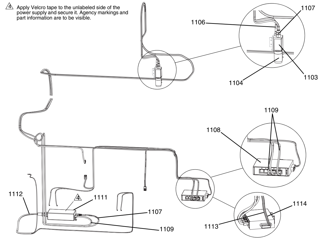
FIG. 33: Vision Camera Kit
