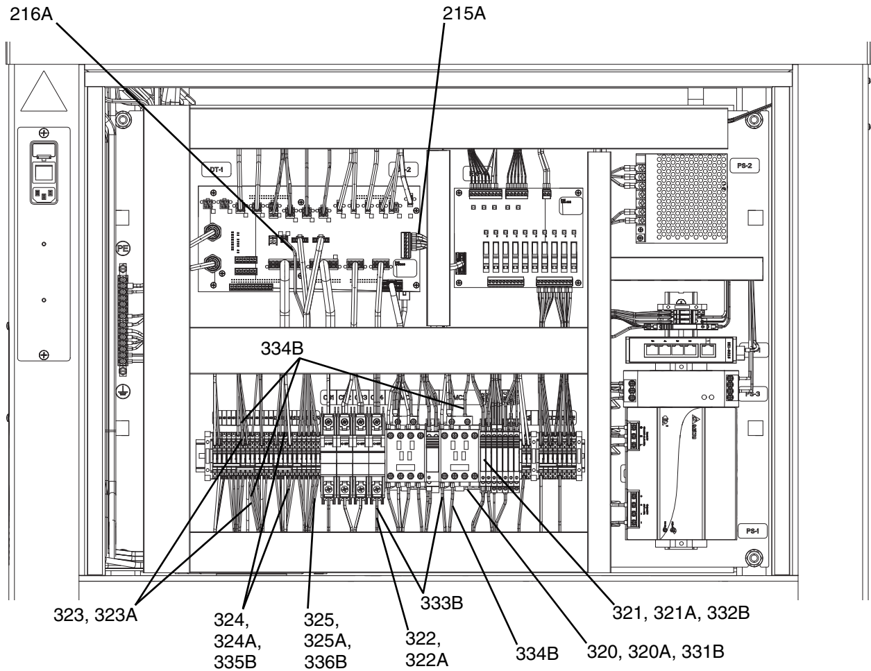
FIG. 39: Wiring Connections
