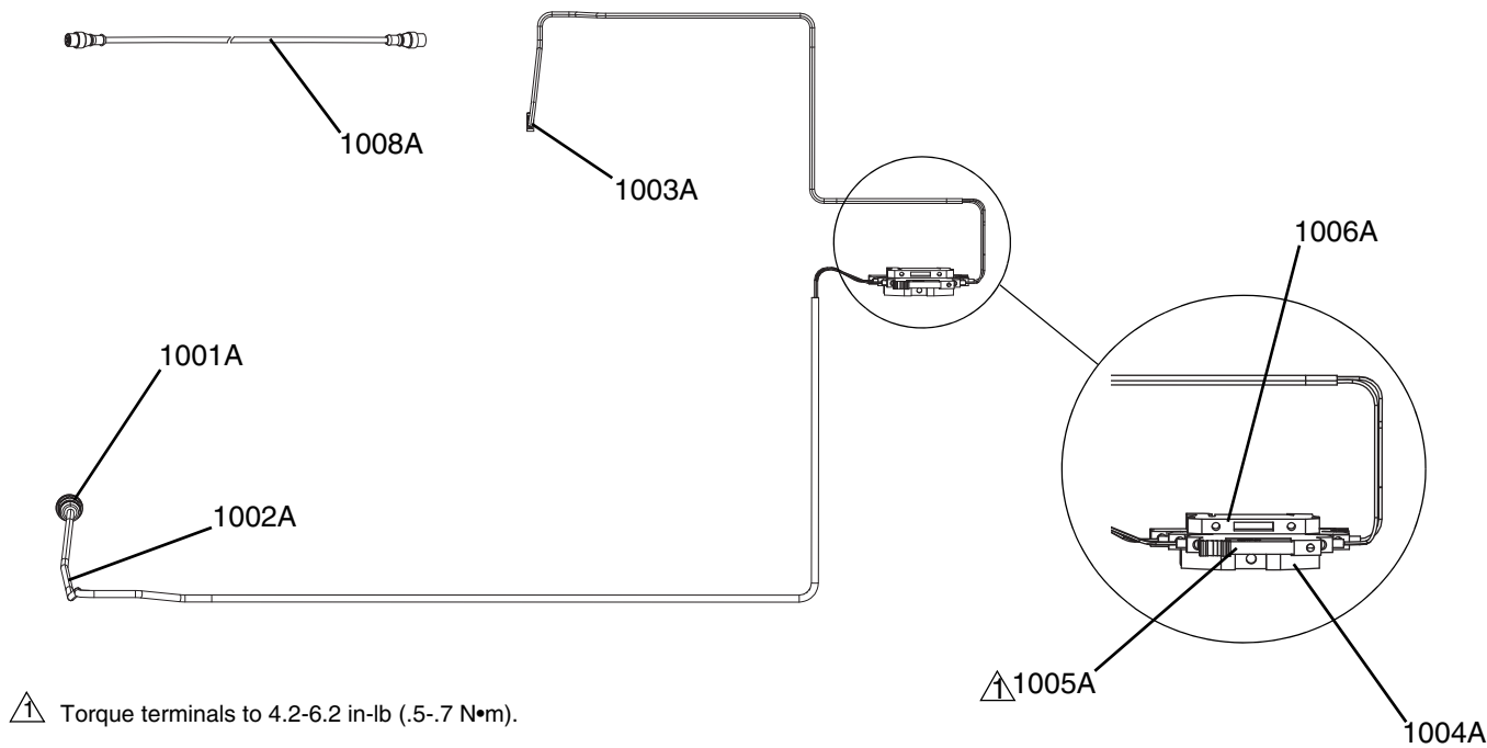
FIG. 32: PCF and HFR Connections
