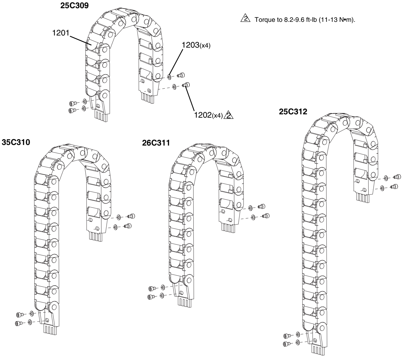
FIG. 34: Cable Tracks
