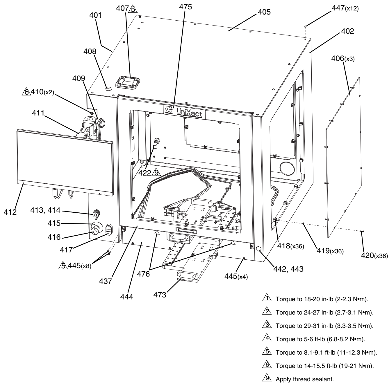
FIG. 20: C-300 Guard Assembly 25C009
