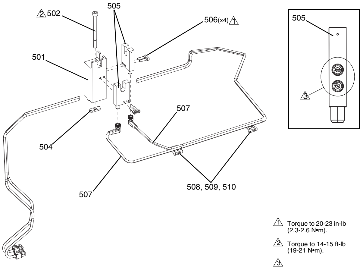
FIG. 26: Needle Find Sensor
