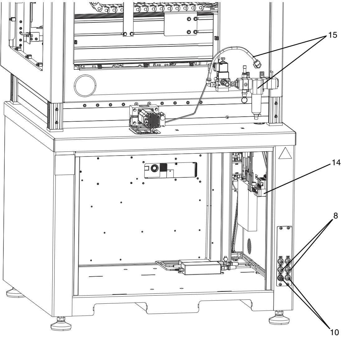
FIG. 3: C-300 and C-500 System Parts 3 (Rear View)
