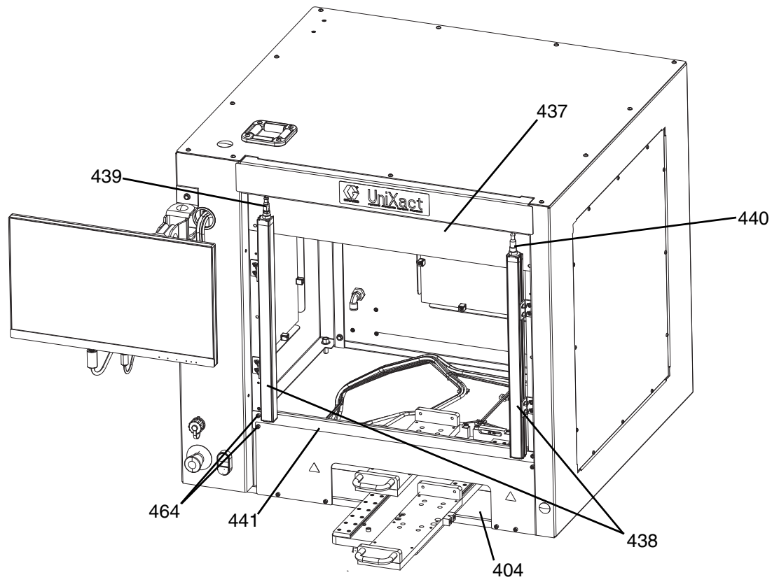
FIG. 21: C-300 Guard Assembly 25C008
