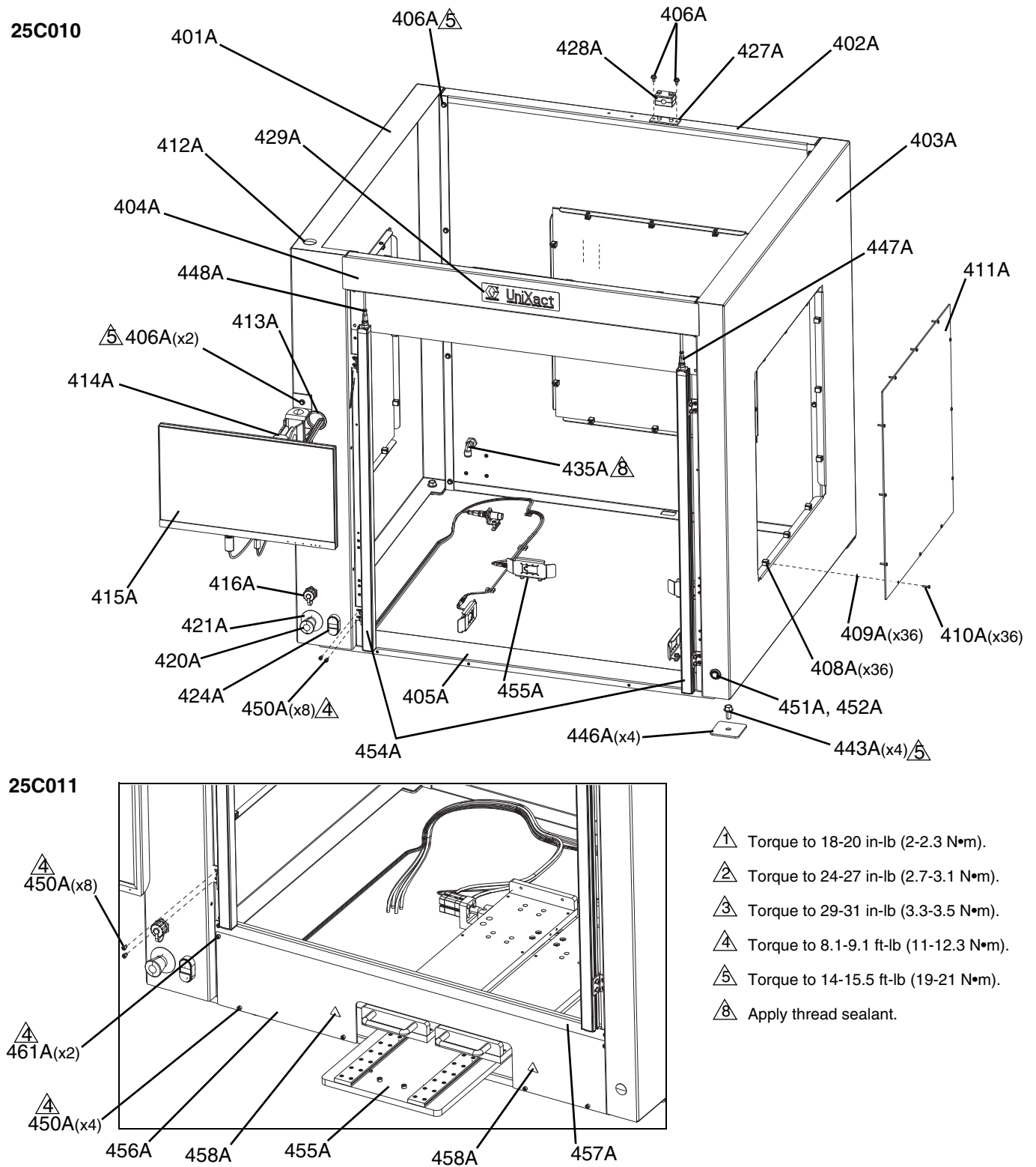
FIG. 24: C-500 Guard Assemblies
