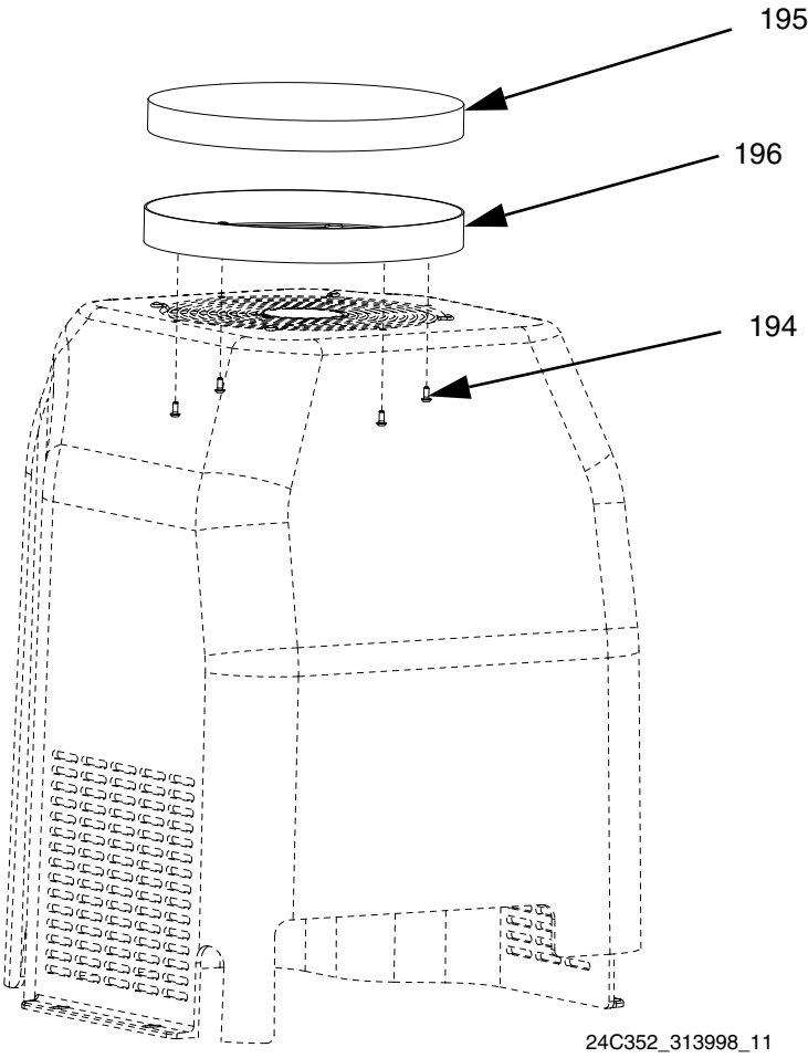
FIG. 16: Base Machine, Image 6 of 6
