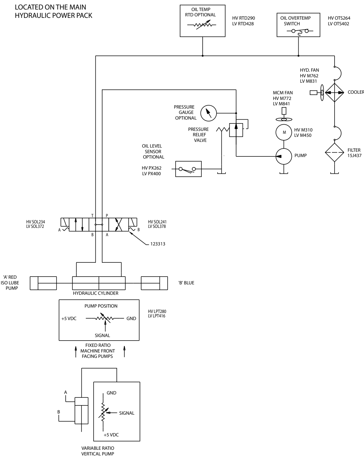
FIG. 37: DC Hydraulic Power Pack Logic Drawing, Page 1 of 1
