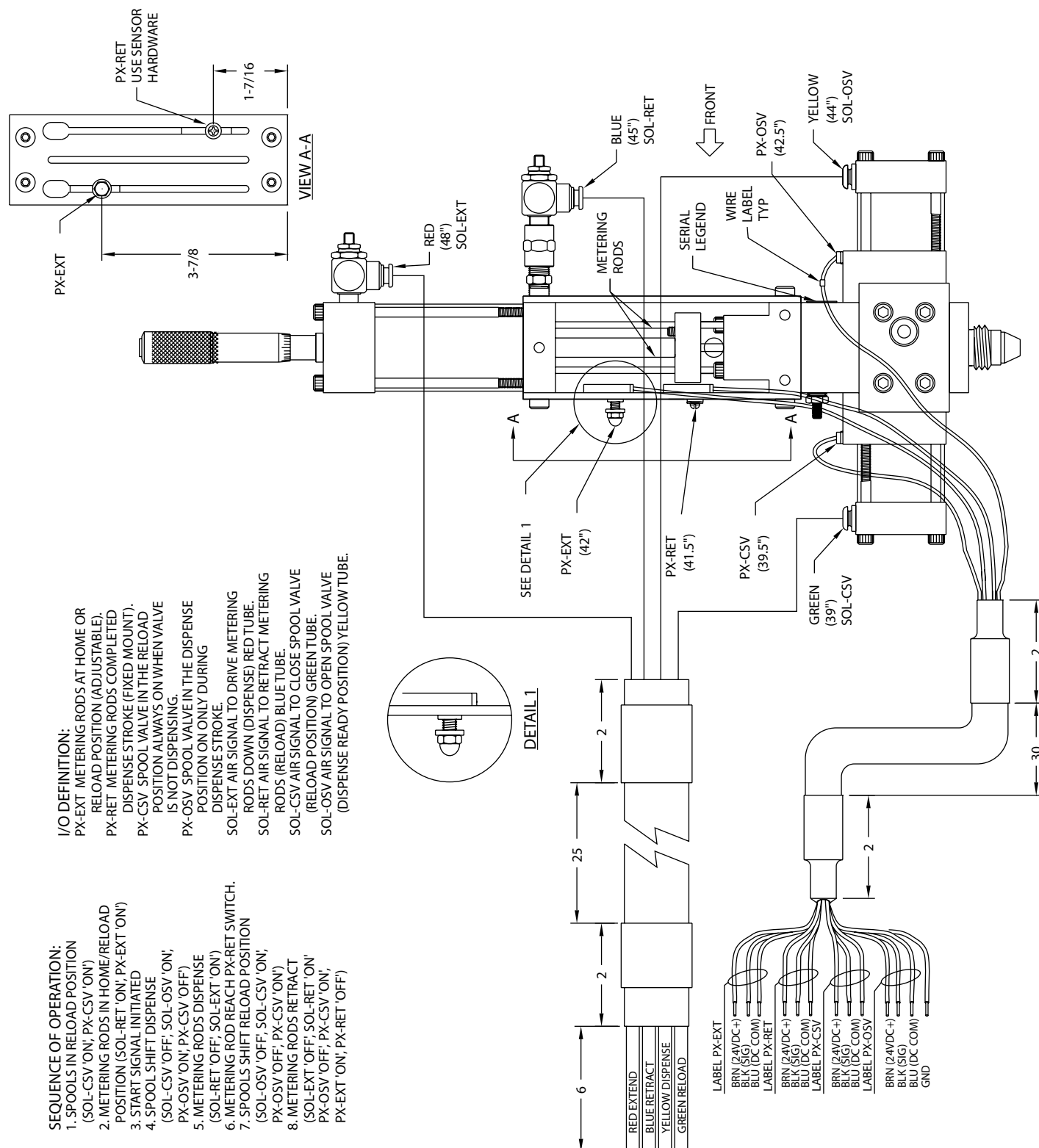
FIG. 13: Micrometer PD44 Metering Valve Electrical Requirements
